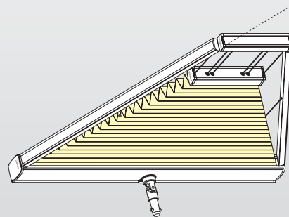
Tensioned blind with crank operation, top track, wire tensioning and two-sided sloped hanging (up to 70 mm in the vertex)
