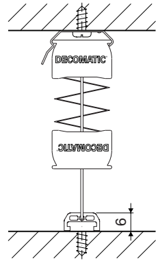
Cord guiding with tension cord fixing
