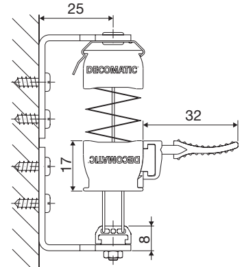
Blind with two hangings
