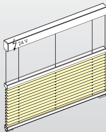
Free-hanging blind with motor operation, variable hanging and cord guiding
