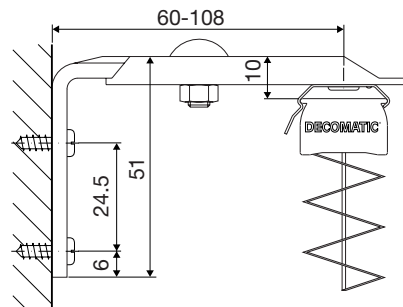
Standard profile with face fix bracket, 60-108 mm
