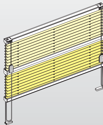
Free-hanging blind with two cord operation units, two hangings and cord guiding
