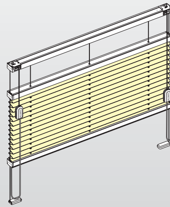
Free-hanging blind with two cord operation units, variable hanging and cord guiding
