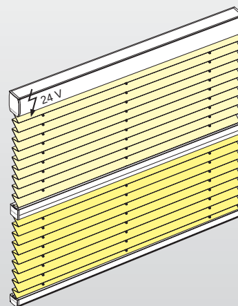
Free-hanging blind with motor operation and two hangings
