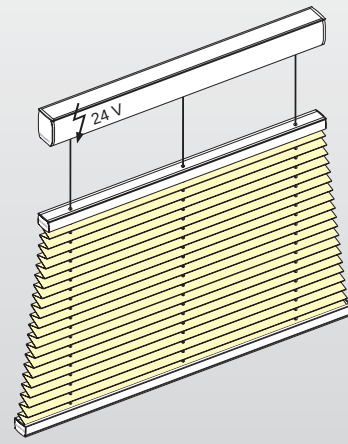
Free-hanging blind with motor operation and two-sided sloped hanging (up to 0.15 m each side)
