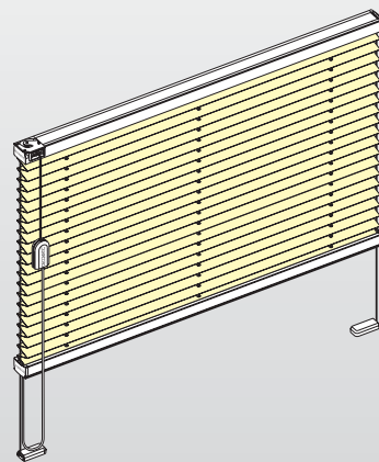
Free-hanging blind with cord operation and cord guiding
