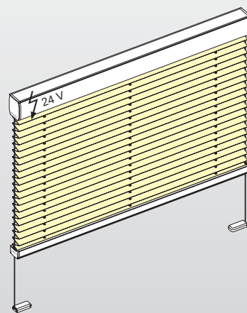
Free-hanging blind with motor operation and cord guiding
