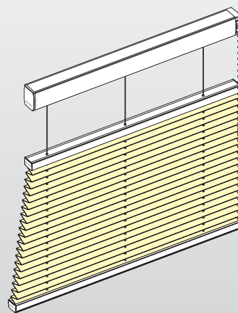
Free-hanging blind with chain operation and a one-sided sloped hanging (up to 0.15 m)
