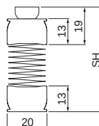
SH (a) Standard up to W = 0.70 m
