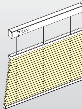
Free-hanging blind with motor operation and one-sided sloped hanging (up to 0.15 m)
