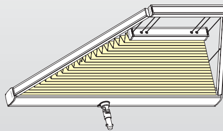
Tensioned blind with crank operation, top track, wire tensioning and two-sided sloped hanging (up to 0.70 m each side)
