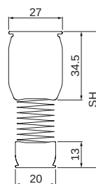
SH (a) Standard
