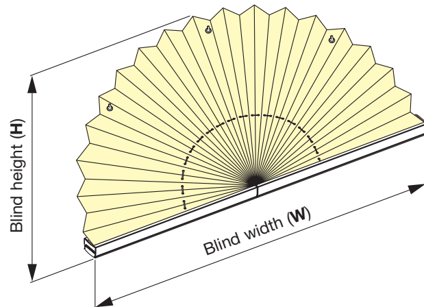
Blind width = 2 x blind height
