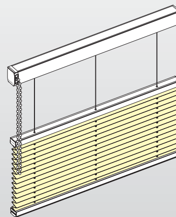
Free-hanging blind with chain operation and variable hanging
