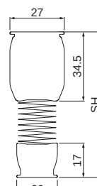
SH (b) Optional with tension profile
