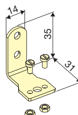
Wall fixing with tension cord angle
