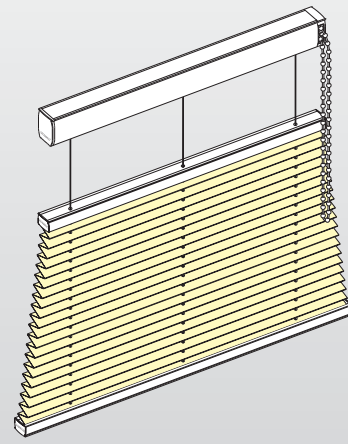
Free-hanging blind with chain operation and a two-sided sloped hanging (up to 0.15 m each side)
