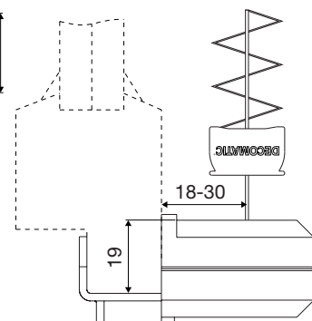
Cord fixation with block holder
