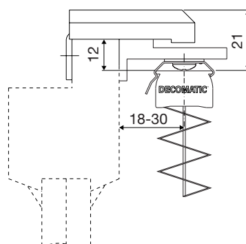
Standard profile with block holder + clip
