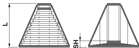
Blind length L
