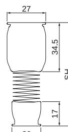
SH (b) Optional with tension profile
