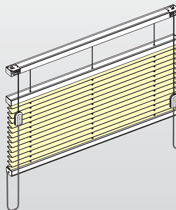
Free-hanging blind with two cord operation units and variable hanging
