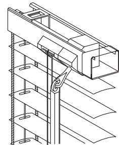
Type 5 - interior blind with worm gear
