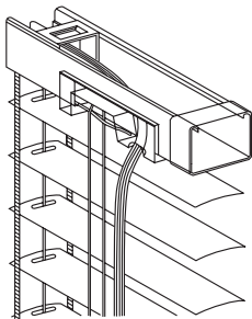
Type 3 - interior blind with flexible joint
