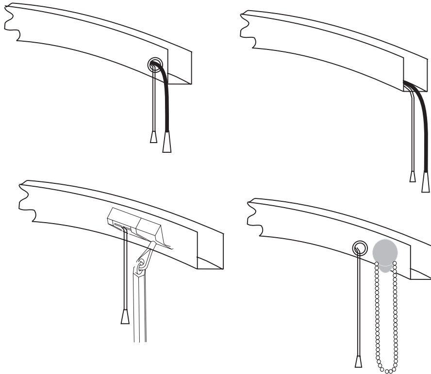
Arch blind controls
