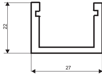
Arch blind head rail - dimensions
